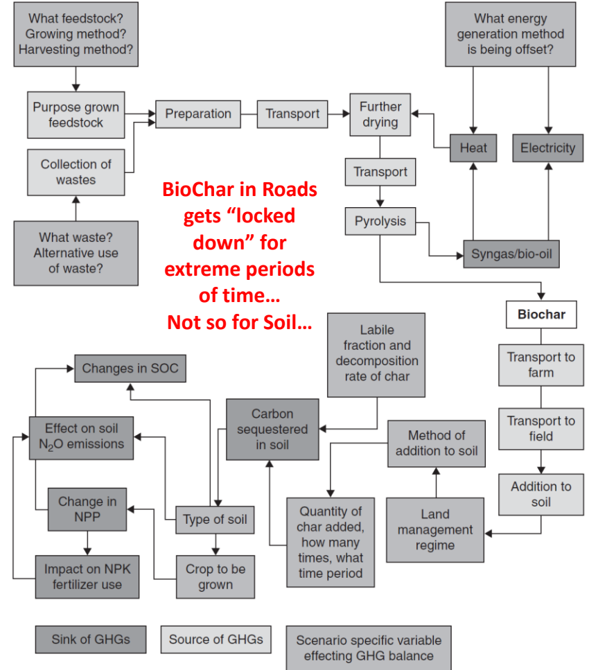
Life Cycle Analysis of Biochar
